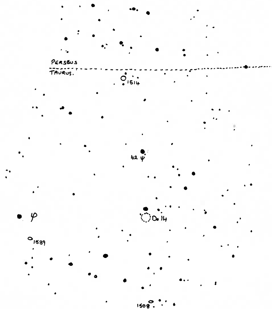
FIG. 6 - NGC 1514 AND DeDz 14
